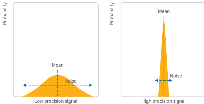
Fig 2 | Bayesian statistics operate on the basis of input probability density functions containing both a mean value and a precision (inverse variance or noise)
